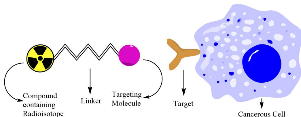
Figure 1. Graphical representation of Radiopharmaceuticals.
