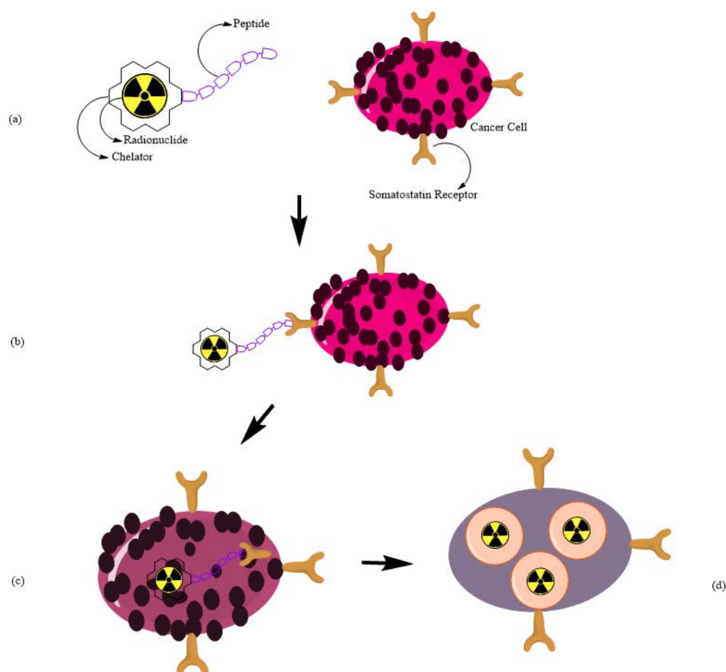
Figure 4. Schematic representation of Peptide Receptor Radionuclide Therapy (PRRT) mechanism; (a) on the left, radiopharmaceutical composed of radionuclide, chelator and a peptide; on the right a generic cancer cell exhibiting a somatostatin receptor; (b) binding between the radiopharmaceutical and the somatostatin receptor; (c) internalization of the radiopharmaceutical in the cancerous cell; (d) radioactivity of the radionuclide in the target cell.
