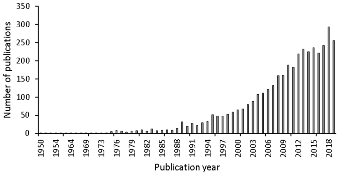
Figure 2. Publication trend on rare actinomycetes from 1950 to 2019. The data were retrieved from PubMed. The search term “Rare actinomycetes” was used to extract the data from PubMed.
