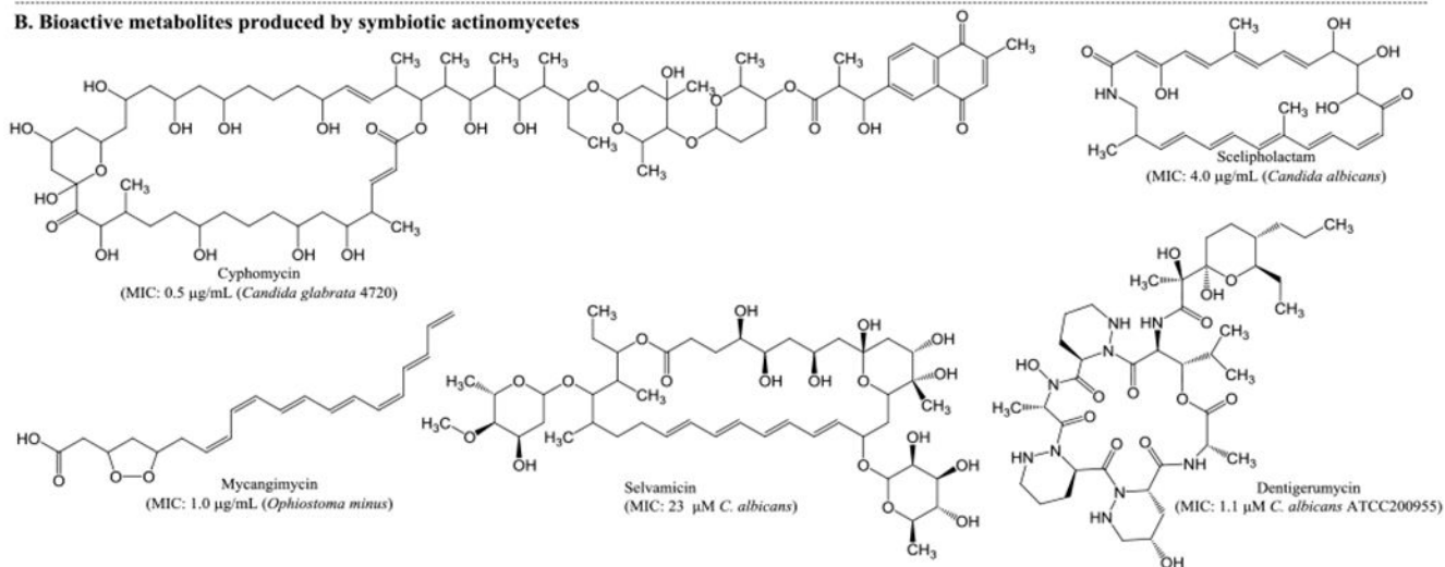
Figure 4. Representative examples of bioactive metabolites isolated from actinomycetes retrieved from the unique environmental origin (a), and symbiotic actinomycetes (b)
