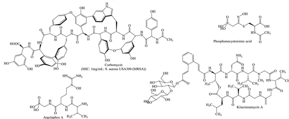
Figure 5. Examples of new metabolites produced by endophytic actinomycetes (A), through co-cultures (B) and genome mining (C)
