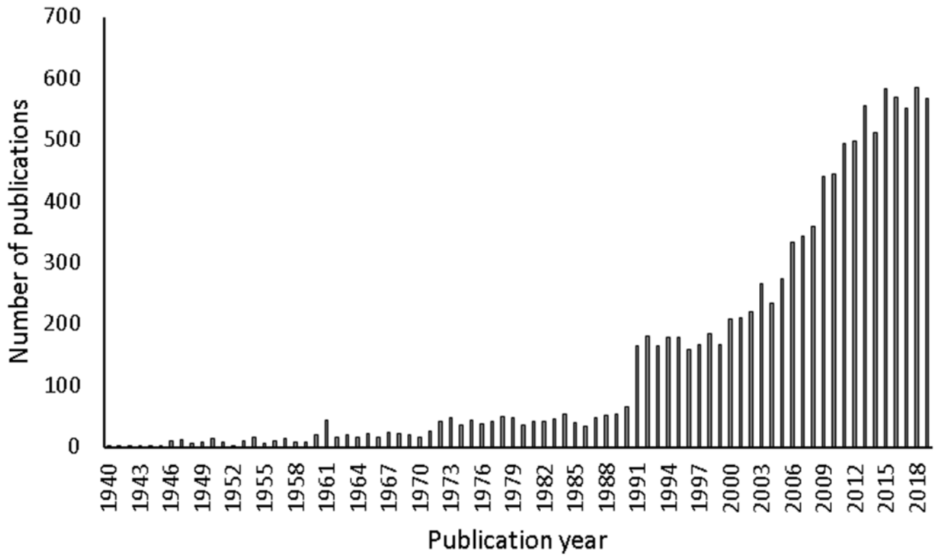
Figure 1. Publication trend on actinomycetes from 1940 to 2018. The data were retrieved from the ISI Web of Science. The search term “actinomycetes” was used to extract the data from PubMed.
