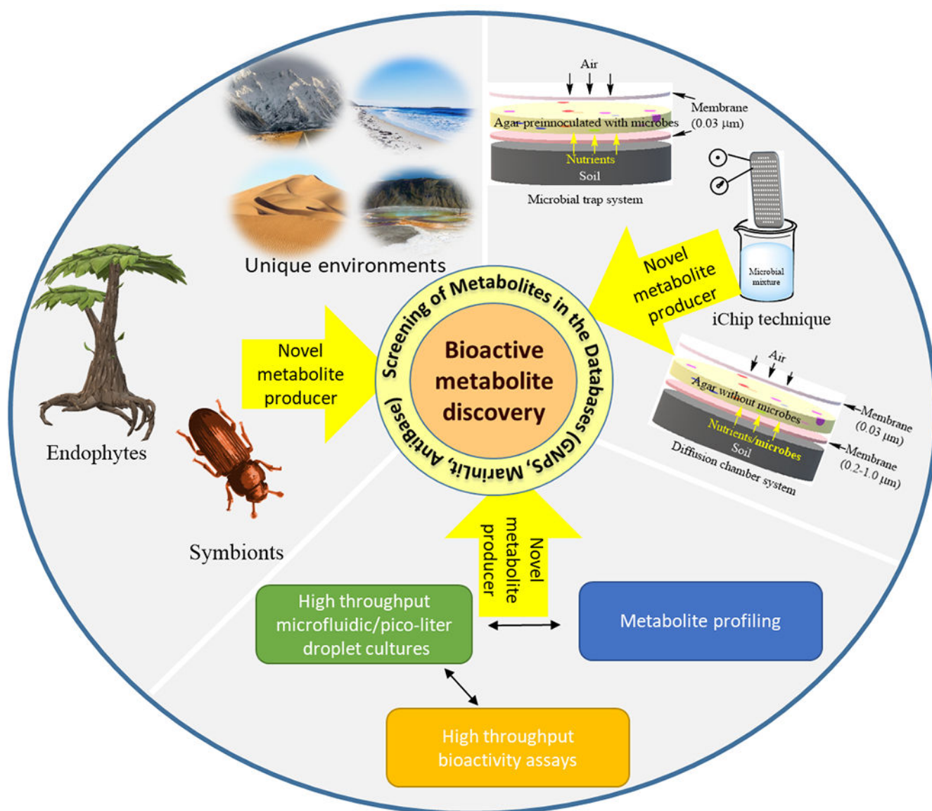
Figure 3. Recently used approaches for the discovery of bioactive metabolites from actinomycetes. While exploration of actinomycetes from unique environments has been conducted for many years, iChip technique, diffusion chamber-facilitated culture, examination of endophytic and symbiotic bacteria, and metabolite profiling-derived discovery of bioactive metabolites represent recently developed approaches. Pictures of natural environments are taken from the creative commons and marked as “dedicated to public domains” (Weblinks: https://search.creativecommons.org/photos/32636618-a8a5-4dcf-81c6-de3ee87f5a6e ; https://search.creativecommons.org/photos/c4b808de-03de-47a8-8c7a-3c8924ec0ff2 ; https://search.creativecommons.org/photos/3be5e8bc-3ac6-4e5c-a9f4-bb717e258998 ; https://search.creativecommons.org/photos/f22282da-d4f9-4400-8051-dfbdf8da0844 )
